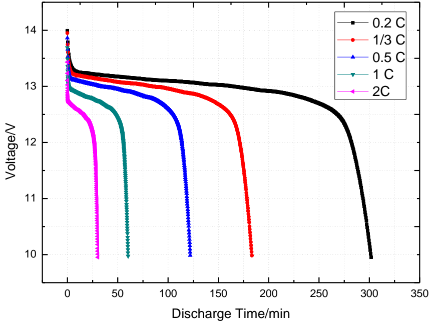
Different Rate Discharge Curve @ 25 °C
