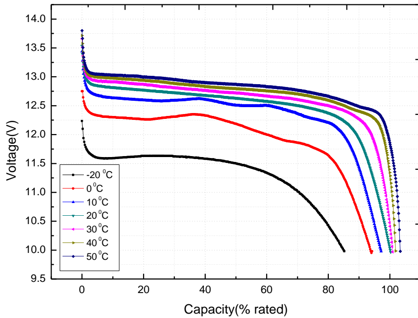
Different Temperature Discharge Curve @ 1C
