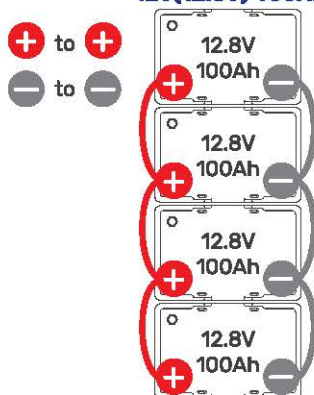
Parallel Connection 12V(12.8V) 400Ah
