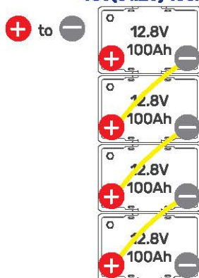
Series Connection 48V(51.2V) 100Ah
