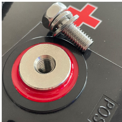
M8 Terminals
