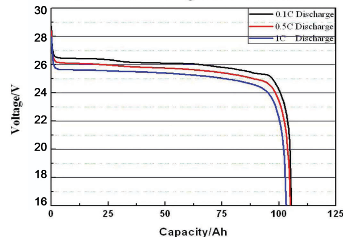
Various Rate Discharge Performance Plot
